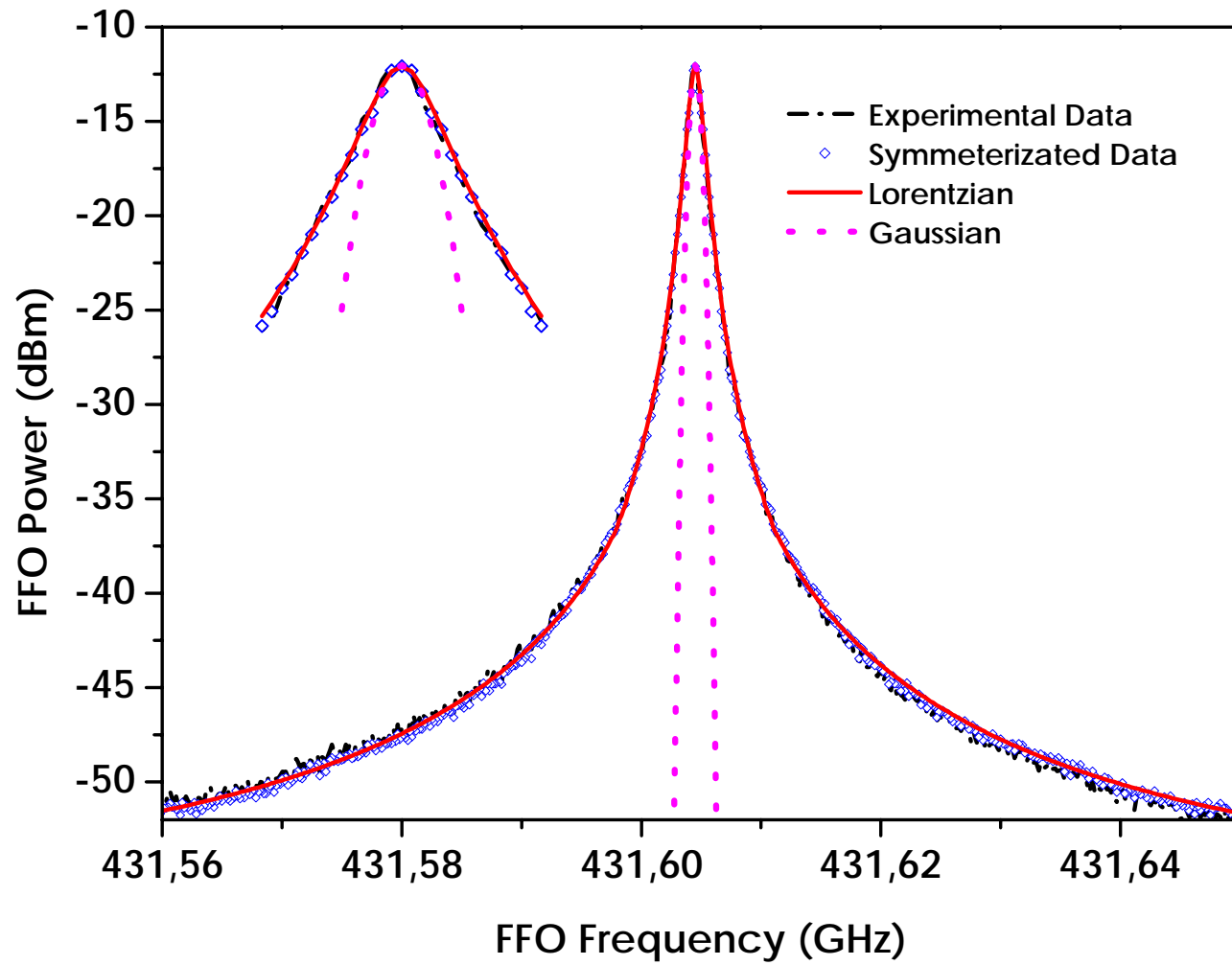
Fig. 15. FFO spectrum measured at 431 GHz ( \mathcal{S}_{AUT} = 1.2 MHz) – dash-dotted line. The symmeterized experimental data are shown by diamonds. Fitted theoretical Lorentzian and Gaussian profiles are shown by solid and dotted lines, respectively. The inset shows a zoom-in on the central peak with the frequency axis multiplied 5 times.
