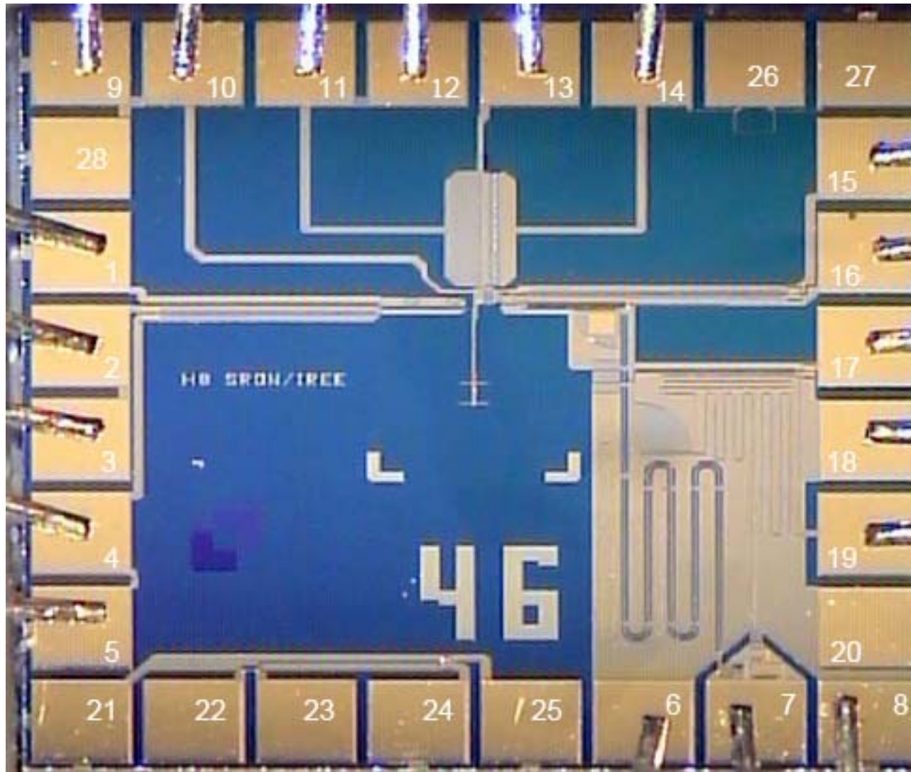
Fig. 18. Microcircuit of the superconducting integrated receiver with phase-locked Josephson oscillator. The chip size is 4 mm by 4 mm.
