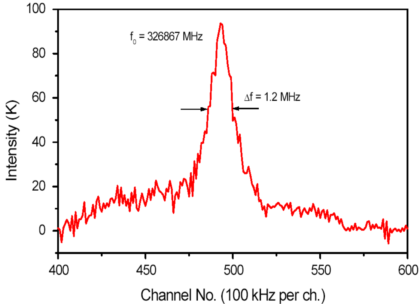
Fig. 23. Spectral line of SO 2 gas at pressure 0.03 mbar detected by superconducting integrated receiver with phase-locked Josephson oscillator (FFO). The data are processed using acousto-optical spectrometer.
