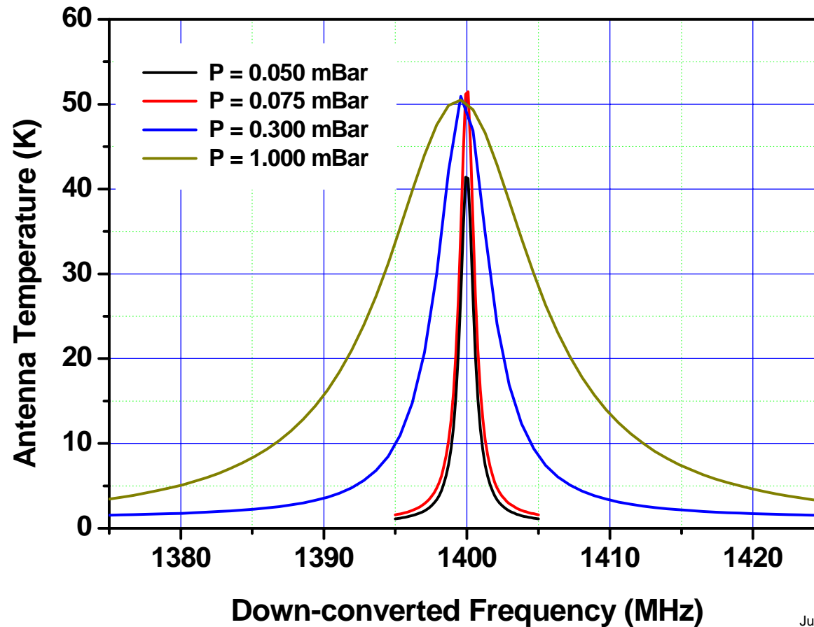
Fig. 22. Effect of broadening of SO 2 gas absorption spectrum at 326.867 GHz measured by PLL superconducting integrated receiver. The Lorentzian fit to experimental data is used.
