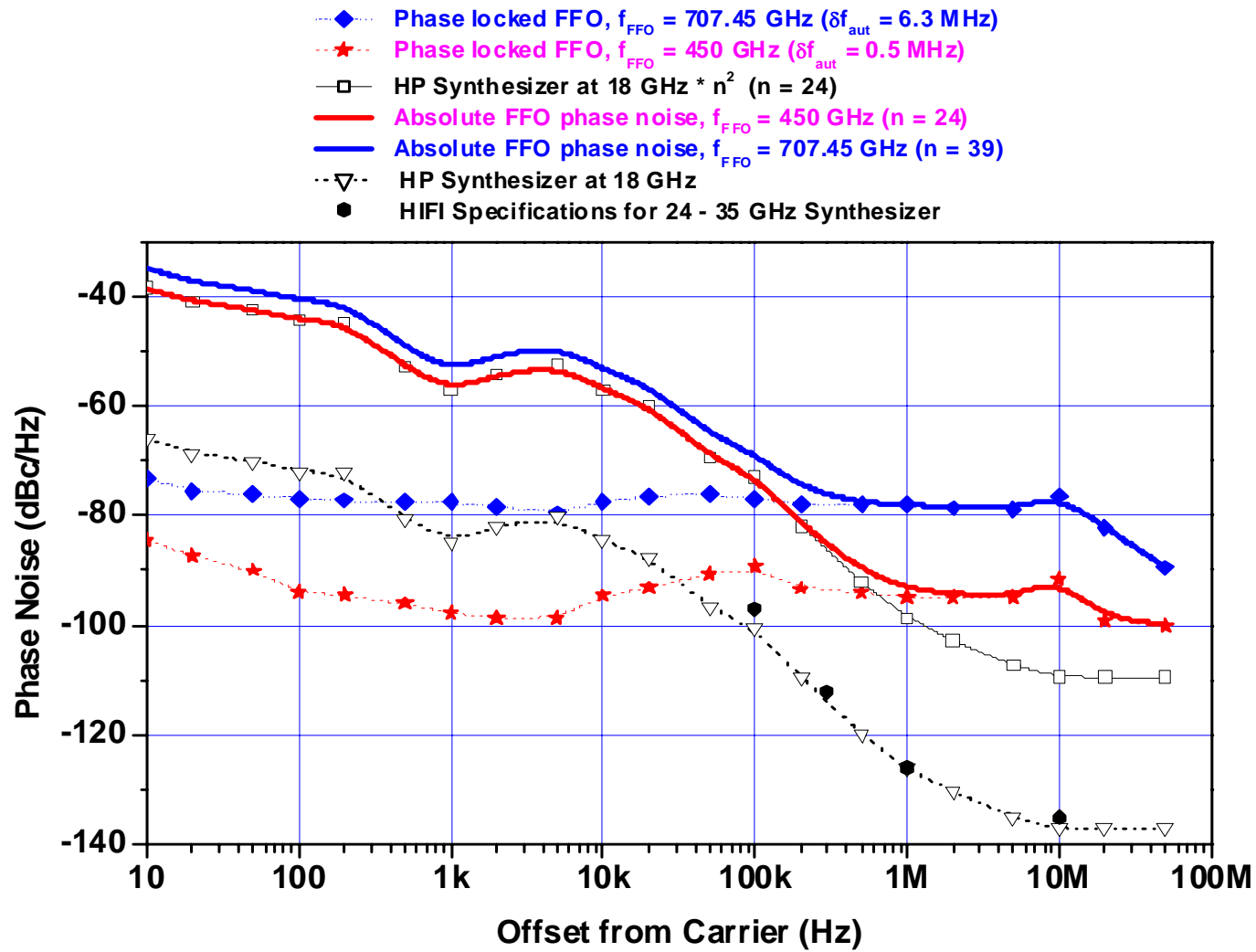
Fig. 17. Phase Noise of the PL FFO. Note that the phase noise at 700 GHz is -80 dBc/Hz at the 1 MHz offset
