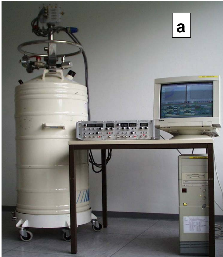
Fig 10. Laboratory Integrated receiver (a). Photographs of exchangeable receiving head (length 76 mm and diameter 32 mm); the input aperture and connectors are seen on the top (b).
