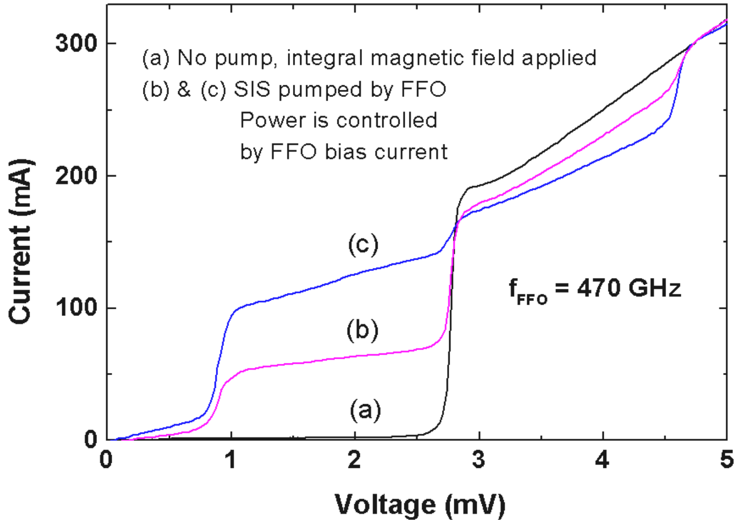
Fig. 13. IVC of the SIS mixer: a) without FFO pump power; b) and c) pumped at two levels ( P_b and P_c ) of FFO power at 470 GHz. The ac Josephson effect is suppressed by a magnetic field.
