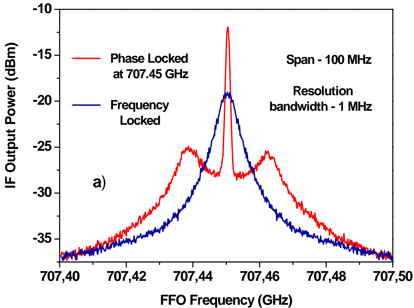
Fig. 16 a. Spectra of the frequency locked and phase-locked FFO operating at 707.45 GHz; the free-running linewidth is \delta f_{AUT} = 6.3 MHz, spectrum analyzer span 100 MHz.
