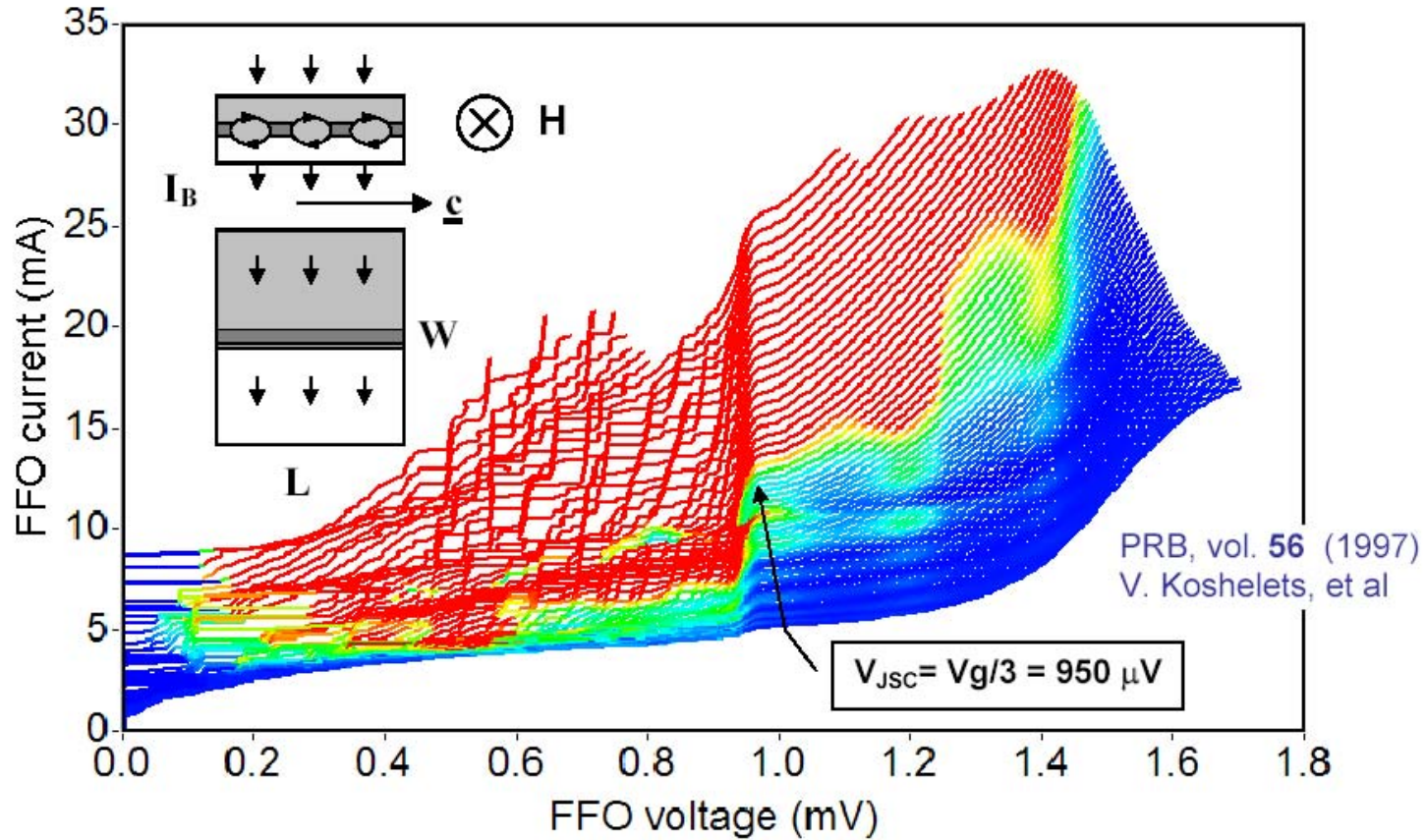
Fig 11. Typical set of IVCs for a Nb-AlO x -Nb FFO recorded with incremented magnetic fields. Each IVC is measured for a fixed control line current, I_{CL} which is then incremented by \Delta I_{CL} \approx 0.5 mA before the next IVC is recorded. Note the abrupt change of the IVC at the boundary voltage V_{JSC} \approx 950 \mu V , above which the voltage and thus the frequency of the FFO increases linearly with \Delta I_{CL} (for fixed bias current I_B ). Insets show the cross section of the long junction with driven vortices (top) and its overlap geometry (bottom).
