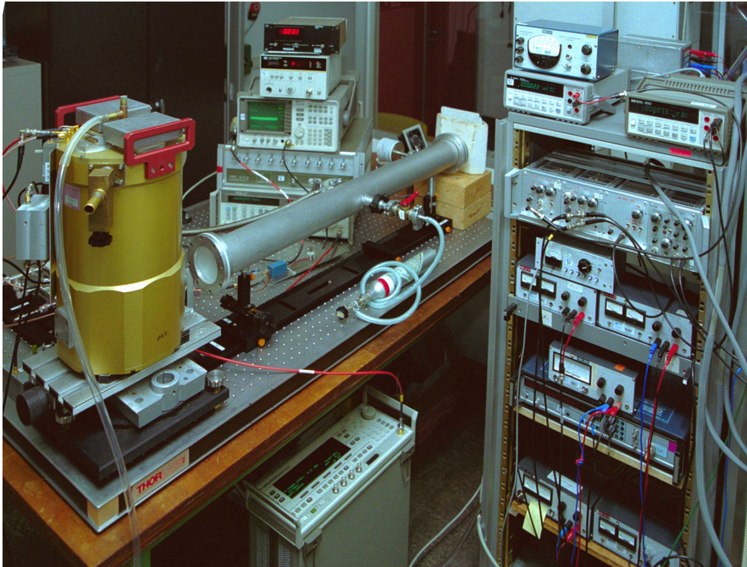
Fig. 20. Gas-cell setup for test of the phase-locked SIR
