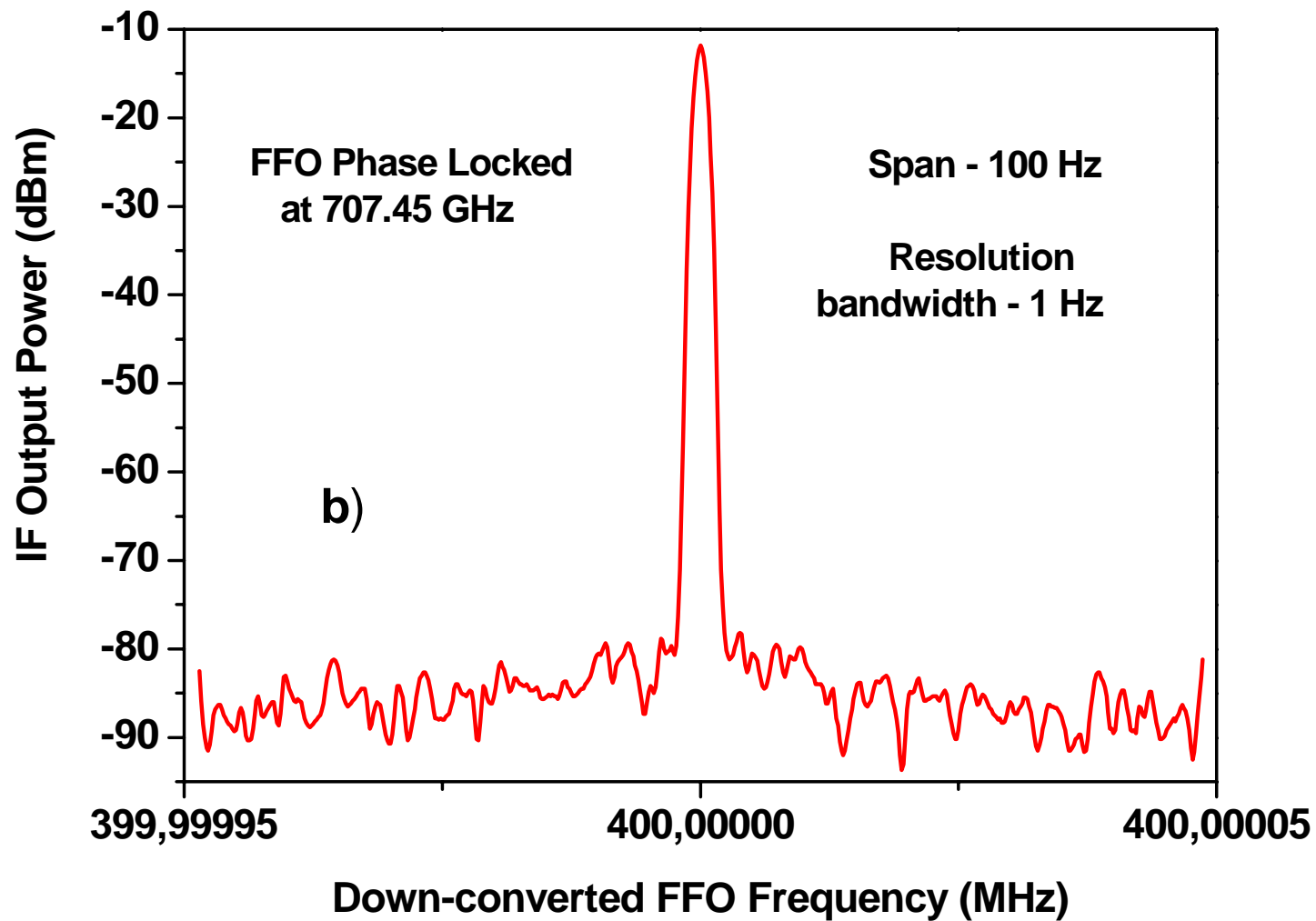
Fig. 16 b. Down-converted spectrum of the FFO phase locked at 707.5 GHz, measured relative to the reference oscillator (spectrum analyzer span 100 Hz, T = 4.2 K)
