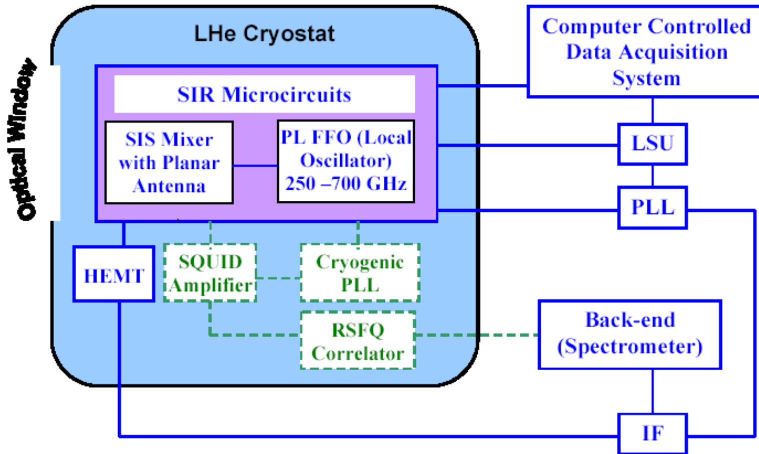
Single-chip Superconducting Integrated Receiver (SIR)
