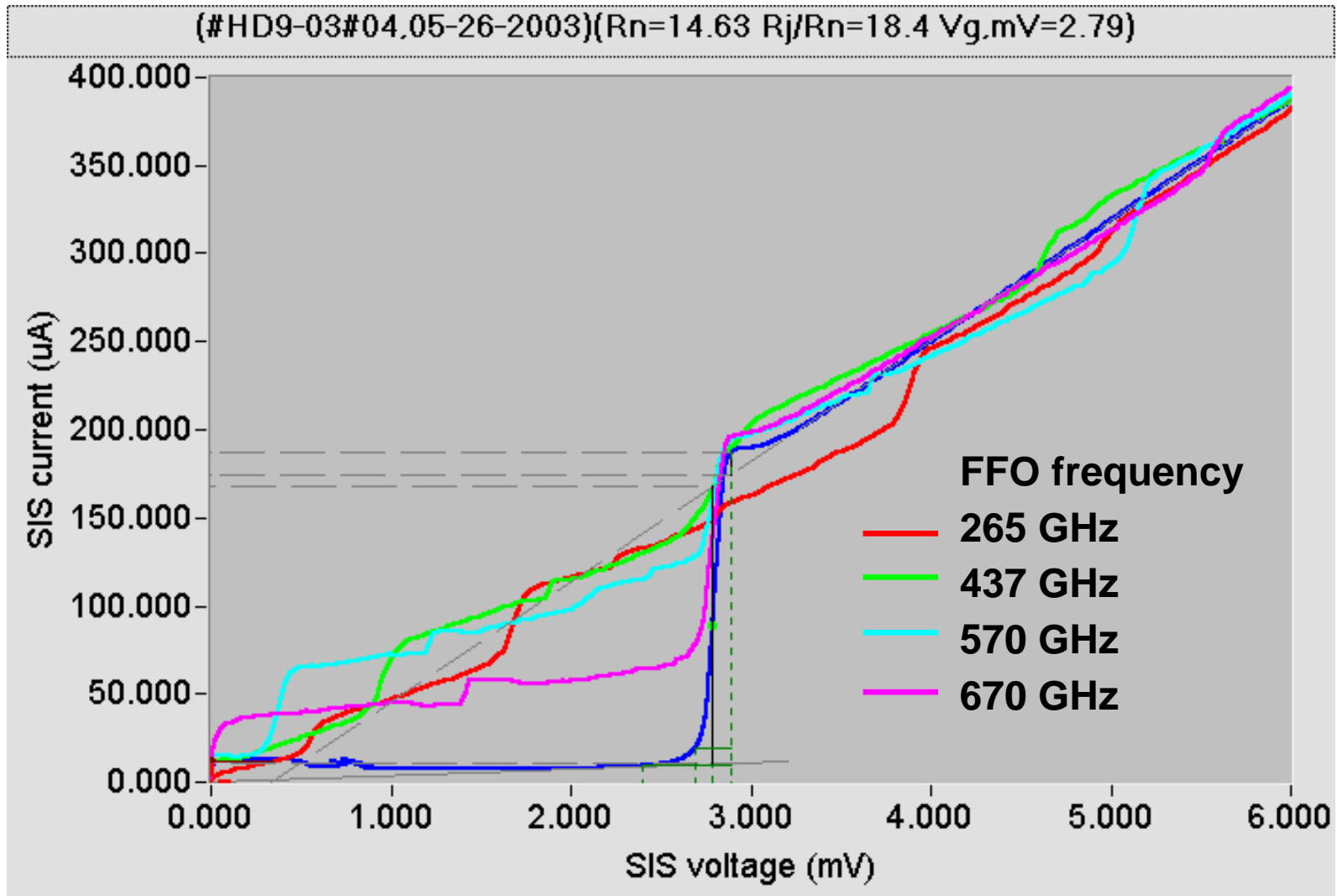
Fig. 12. IVCs of the SIS detector (wide band design) pumped by a FFO at different frequencies 265, 435, 570 and 670 GHz.
