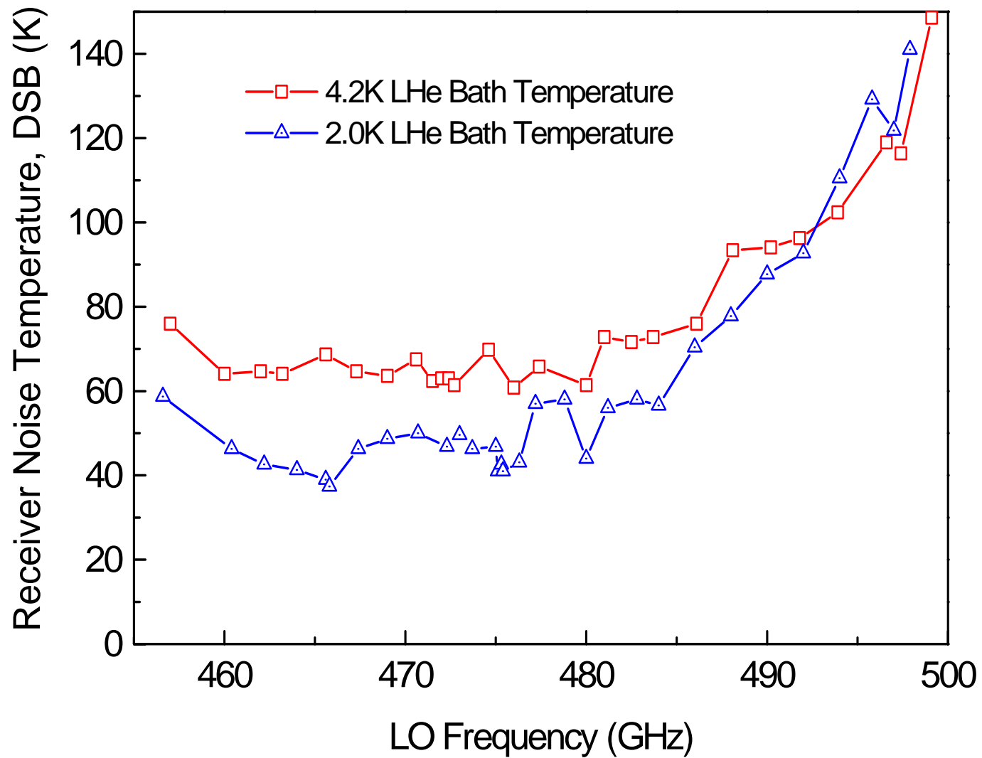
Fig 7. Noise temperature of the quantum-noise-limited Double Dipole Antenna SIS Receiver.
