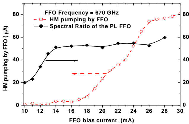
Fig. 3. Dependence of the HM current induced by FFO (HM pumping) and Spectral Ratio after FFO phase locking as a function of FFO bias current. All data measured at FFO frequency of 670 GHz.
