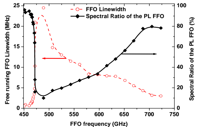
Fig. 4. FFO linewidth and Spectral Ratio of the phase-locked FFO on its oscillation frequency. The data are measured at constant bias current, while the FFO frequency is tuned by the magnetic field (by the control line current).
