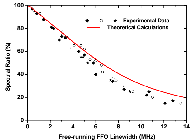
Fig. 2. Spectral Ratio for the phase-locked FFO of different design as a function of free-running FFO linewidth.
